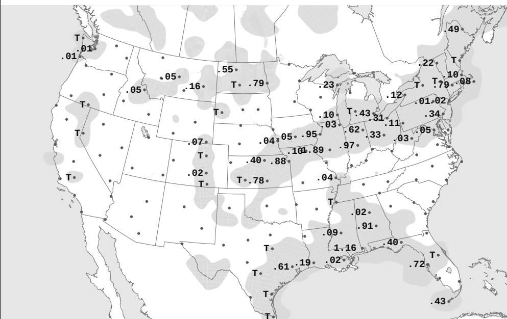
SAT, JUL 26, 2025 24-hour Precipitation Areas and Amounts Ending 7:00 A.M. E.S.T.
