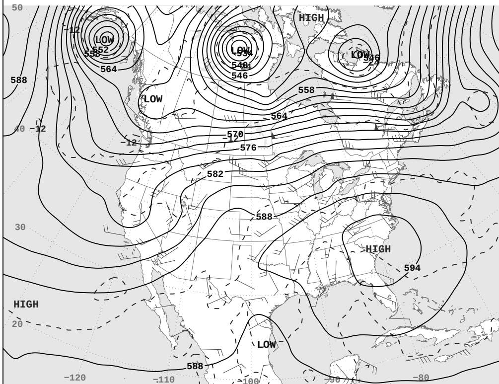
SAT, JUL 26, 2025 500-Millibar Height Contours at 7:00 A.M. E.S.T.
