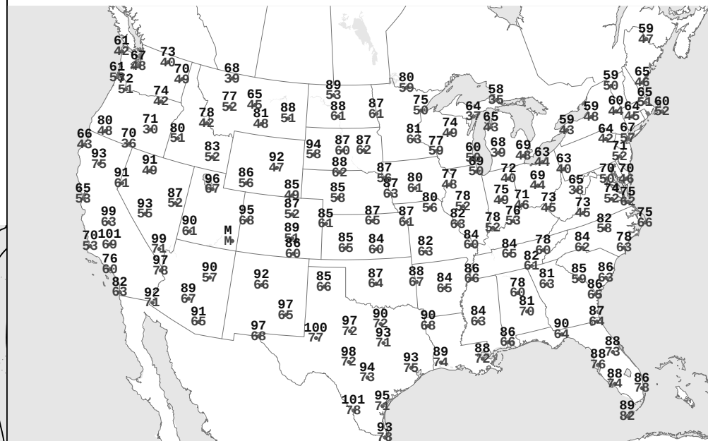
MON, JUN 02, 2025 Highest and Lowest Temperature
