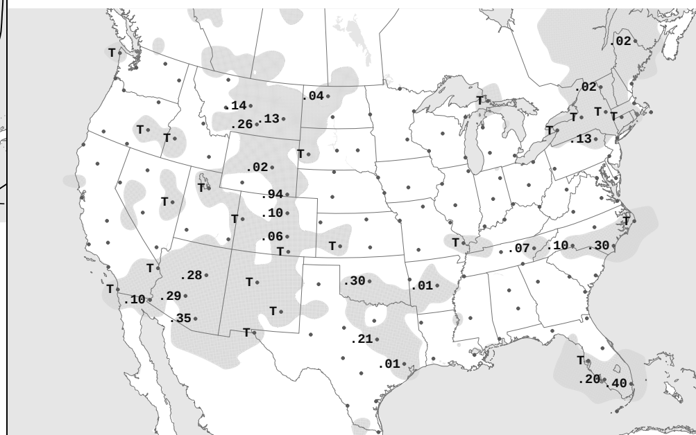
MON, JUN 02, 2025 24-hour Precipitation Areas and Amounts Ending 7:00 A.M. E.S.T.
