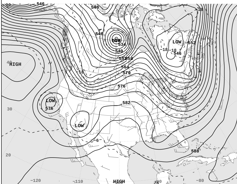
MON, JUN 02, 2025 500-Millibar Height Contours at 7:00 A.M. E.S.T.
